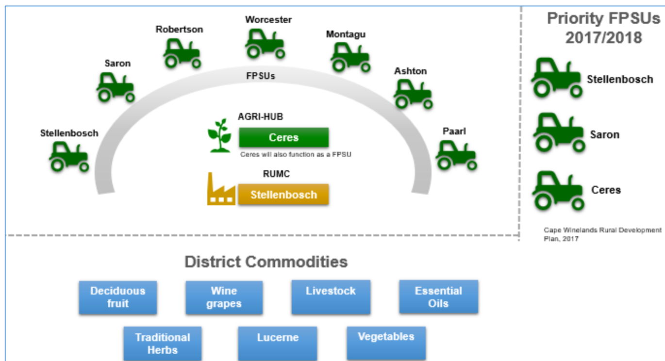
Figure 13: Agri-Park Implementation
