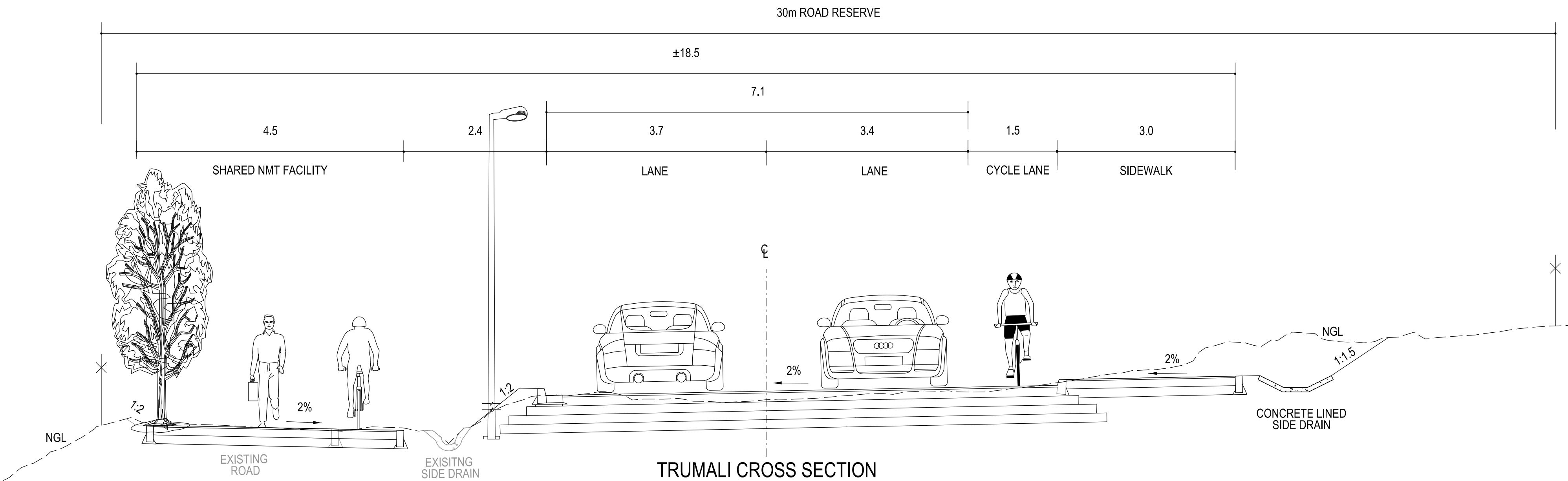
TRUMALI CROSS SECTION OPTION 2
